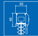
Dimensioni cassonetto Head rail dimensions
