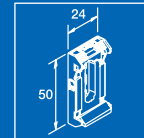
Supporto Push Push bracket
