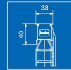
Dimensioni cassonetto Head rail dimensions
