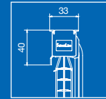
Dimensioni cassonetto Head rail dimensions
