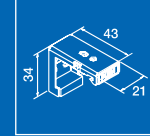
Attacco Push Push bracket
